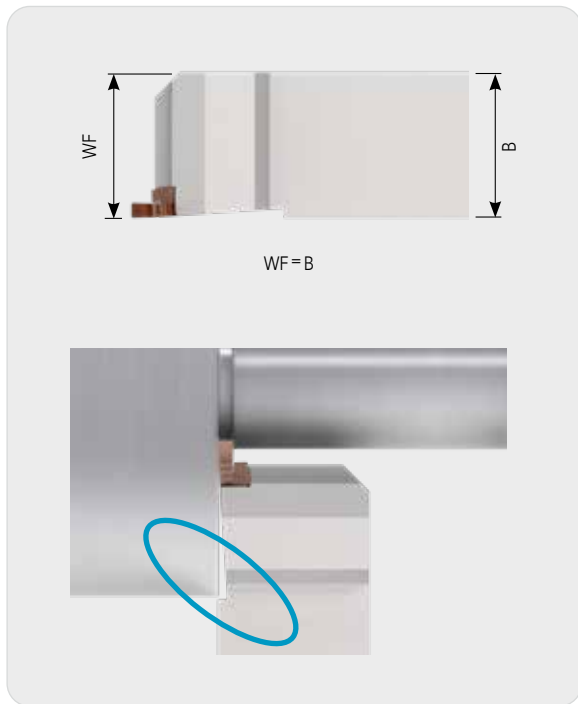
Current holder: Deep depth of cut unavailable
