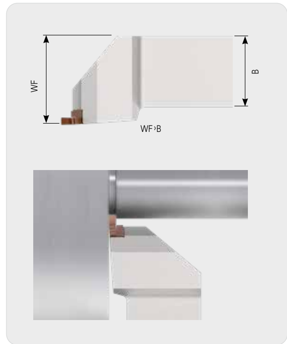
New offset type holder: Deep depth of cut available
